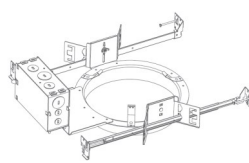
Hanger bar
